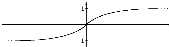
Graph of the function g : \mathbf{R} \rightarrow (-1, 1) given by g(x) = \frac{2}{\pi} \arctan(x) .
